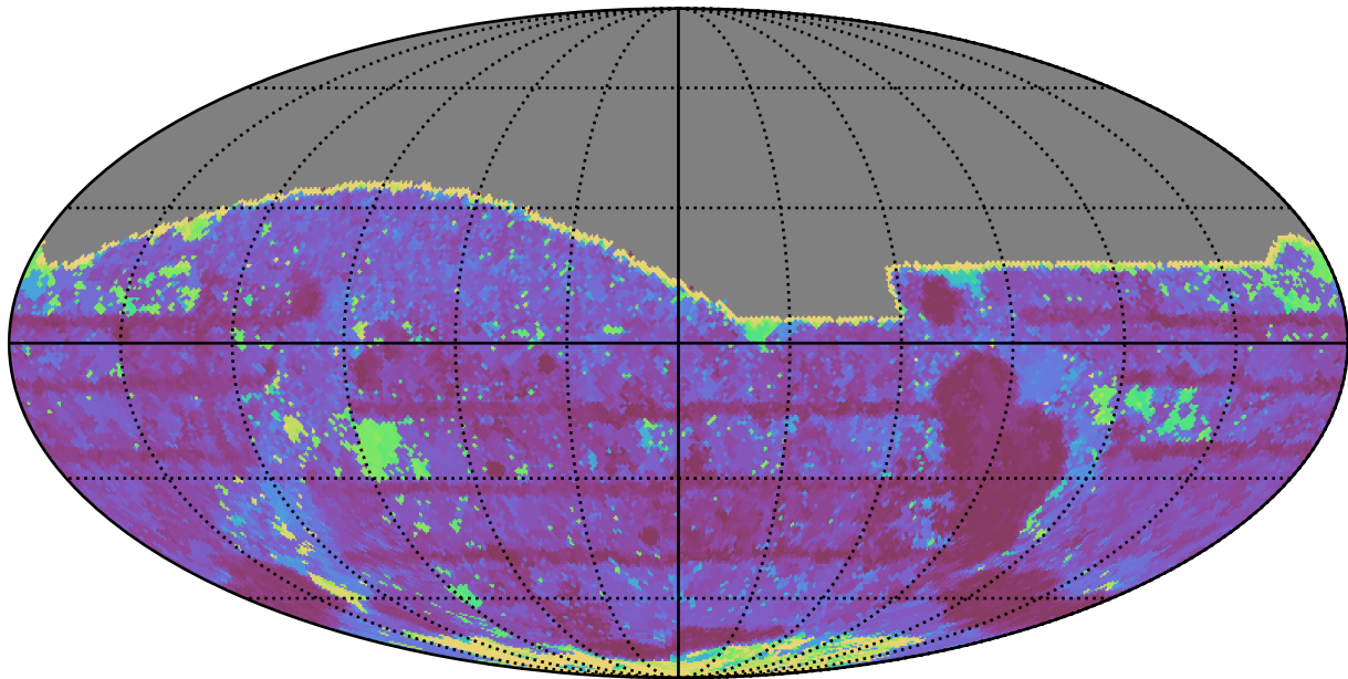
ddf_loaded_fl15_v3.4_10yrs All sky i band: Max Inter-Night Gap
