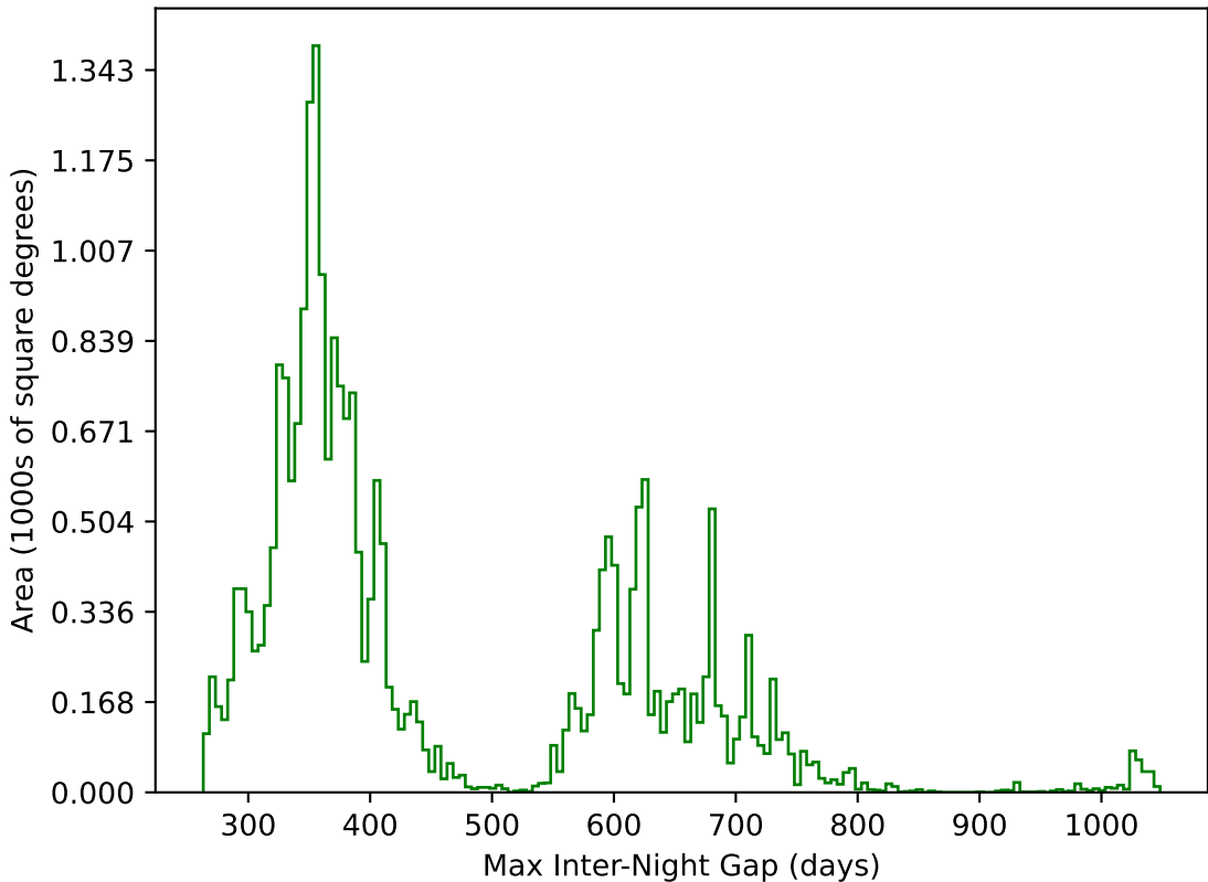
ddf_loaded_fl15_v3.4_10yrs All sky g band: Max Inter-Night Gap
