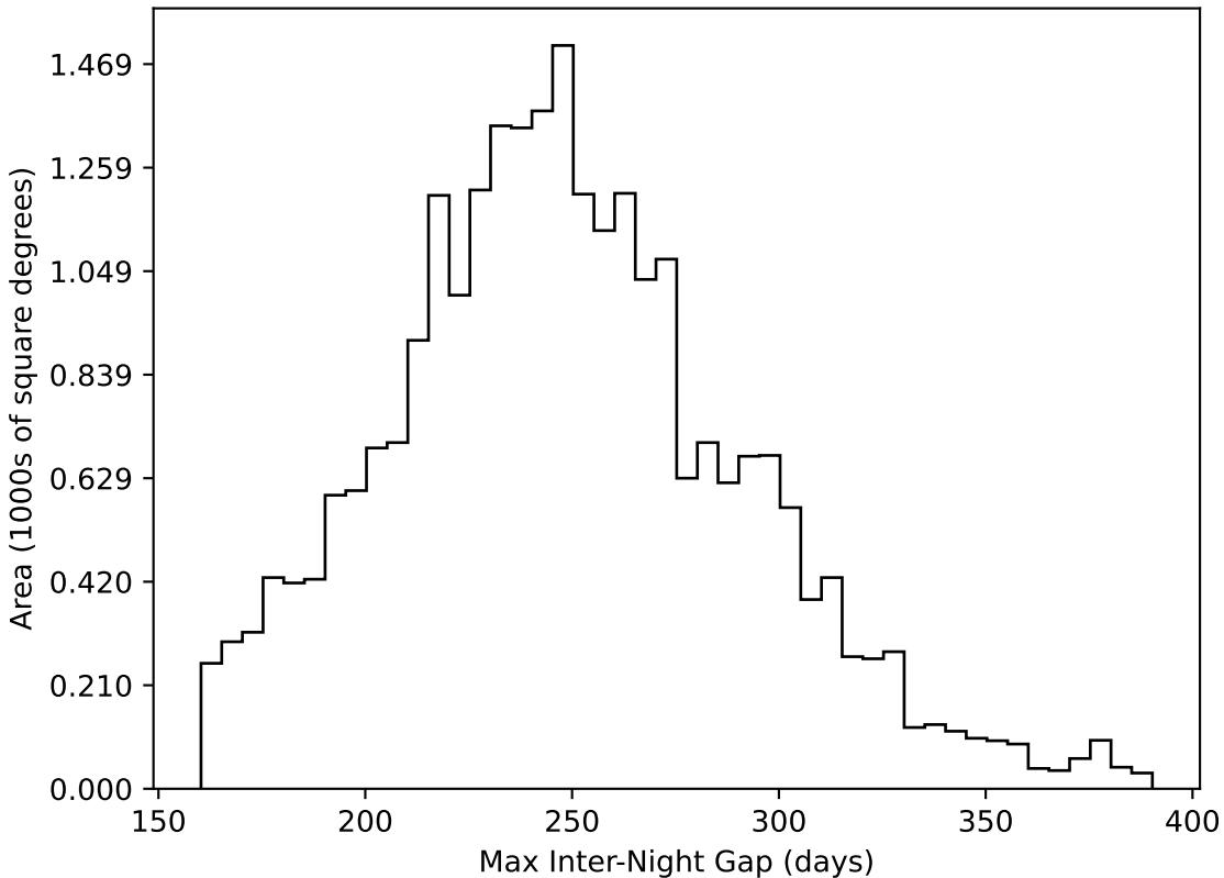
ddf_loaded_fl15_v3.4_10yrs All sky all bands: Max Inter-Night Gap
