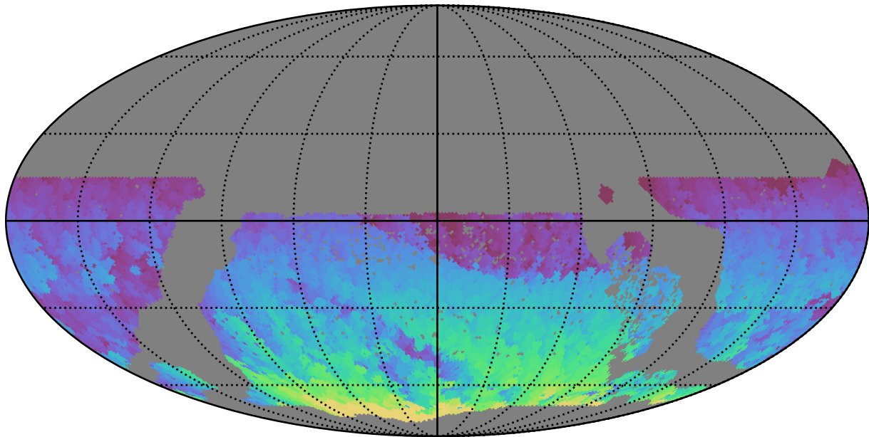
ddf_loaded_fl15_v3.4_10yrs WFD z band: Max HA
