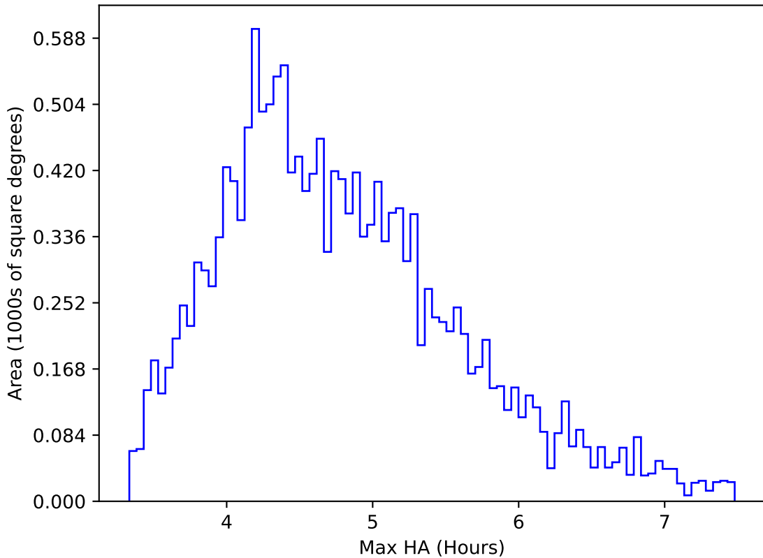
ddf_loaded_fl15_v3.4_10yrs WFD y band: Max HA
