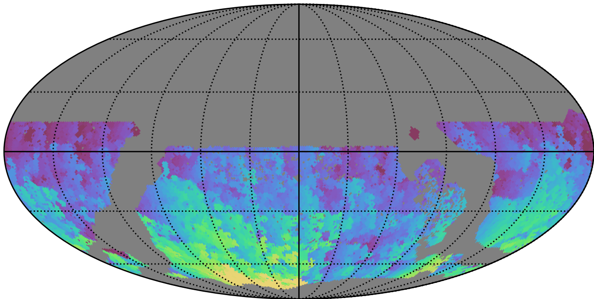
ddf_loaded_fl15_v3.4_10yrs WFD u band: Max HA
