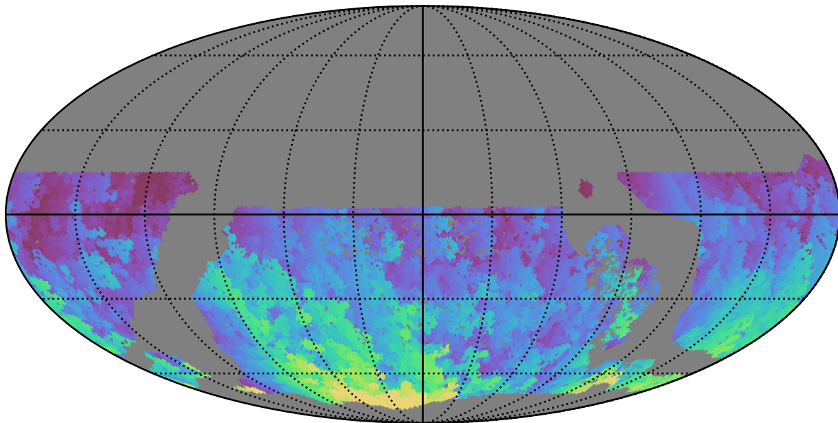
ddf_loaded_fl15_v3.4_10yrs WFD g band: Max HA
