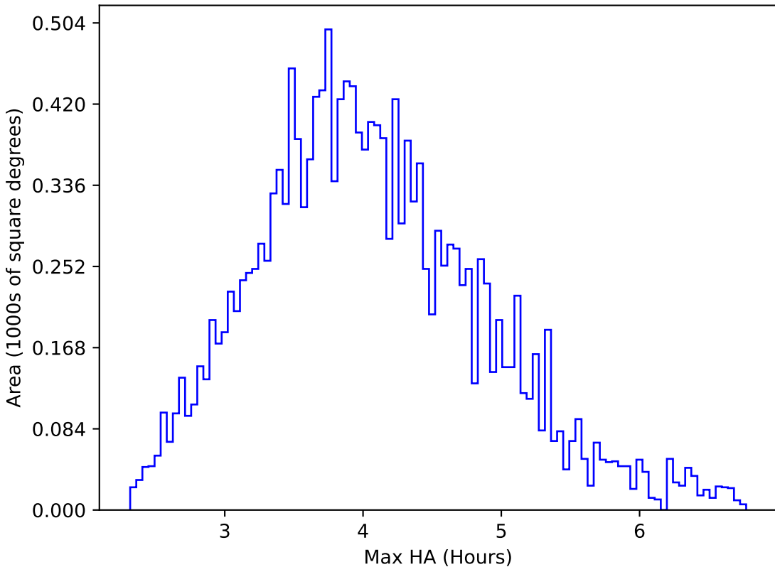
ddf_loaded_fl15_v3.4_10yrs WFD g band: Max HA
