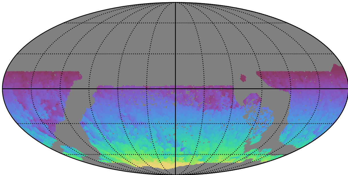
ddf_loaded_fl15_v3.4_10yrs WFD all bands: Max HA
