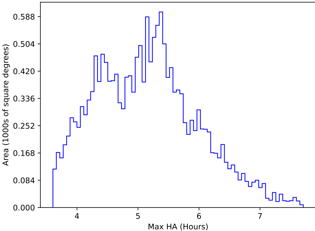
ddf_loaded_fl15_v3.4_10yrs WFD all bands: Max HA
