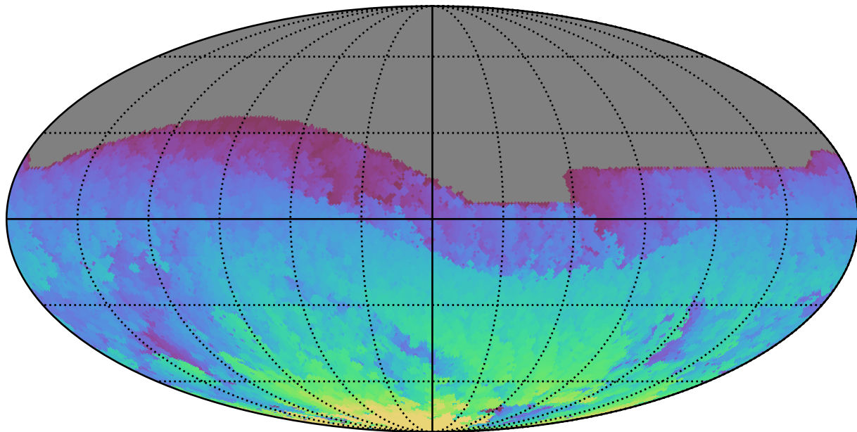
ddf_loaded_fl15_v3.4_10yrs All sky z band: Max HA
