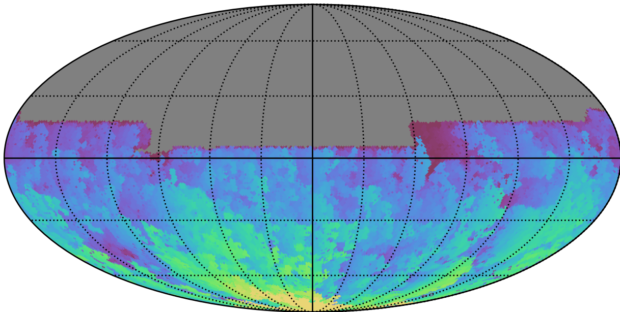
ddf_loaded_fl15_v3.4_10yrs All sky u band: Max HA
