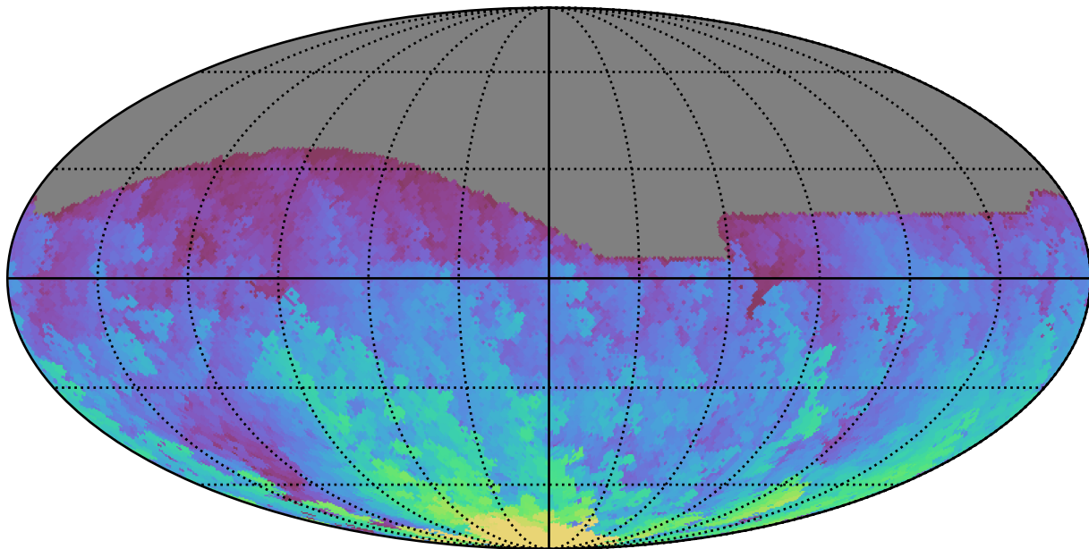
ddf_loaded_fl15_v3.4_10yrs All sky g band: Max HA
