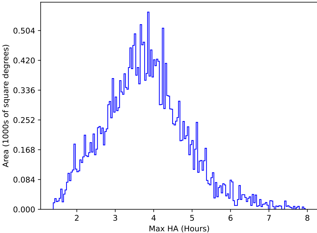
ddf_loaded_fl15_v3.4_10yrs All sky g band: Max HA
