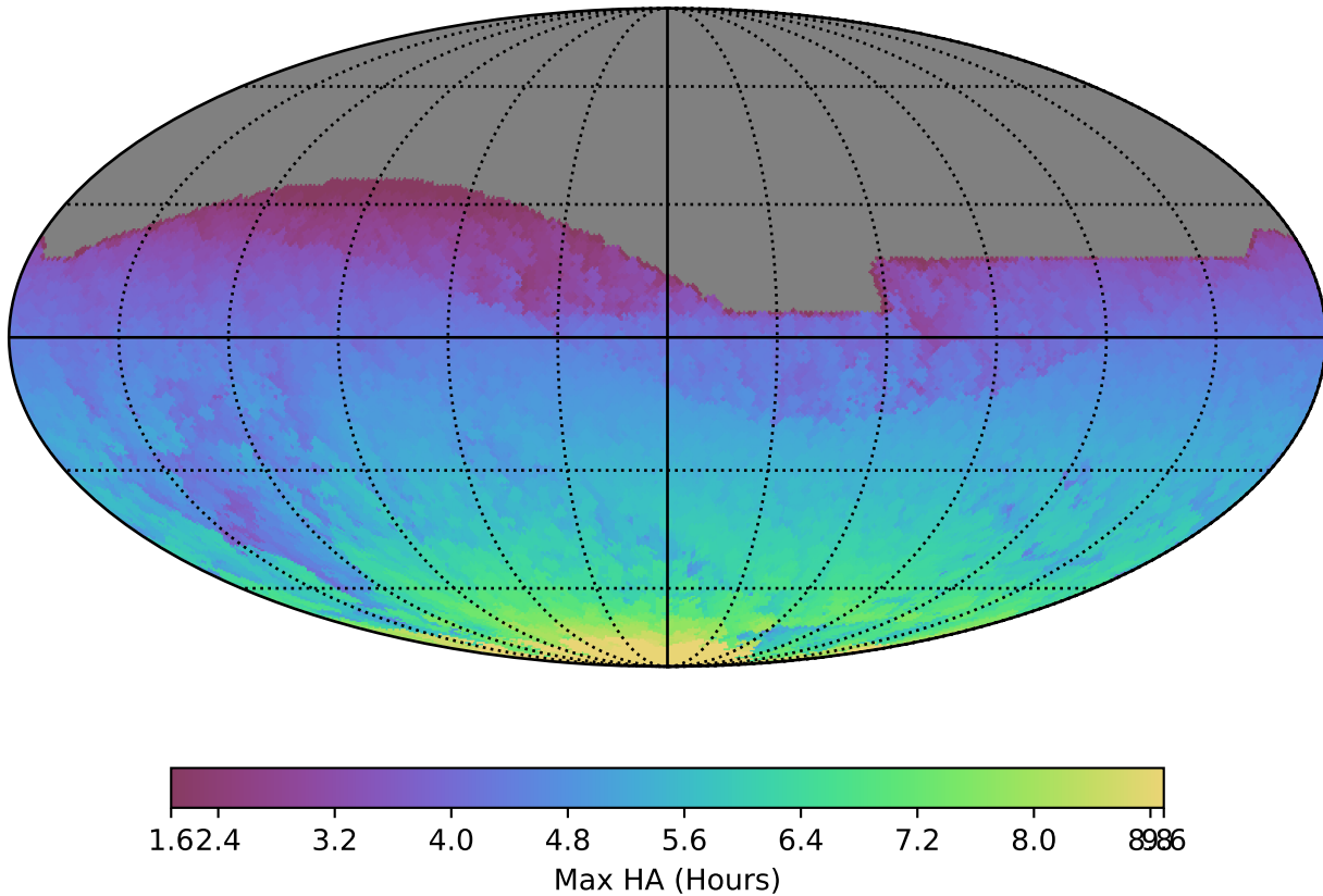
ddf_loaded_fl15_v3.4_10yrs All sky all bands: Max HA
