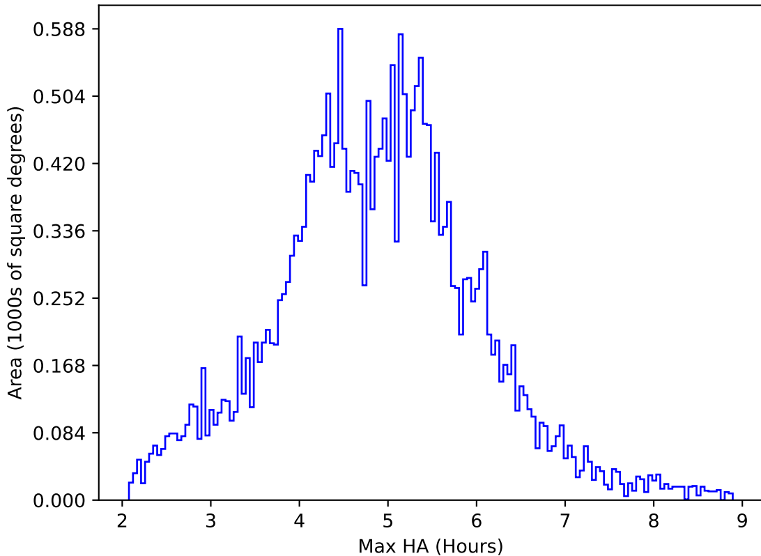
ddf_loaded_fl15_v3.4_10yrs All sky all bands: Max HA
