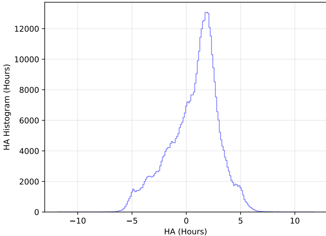
ddf_loaded_fl15_v3.4_10yrs WFD z band: HA Histogram
