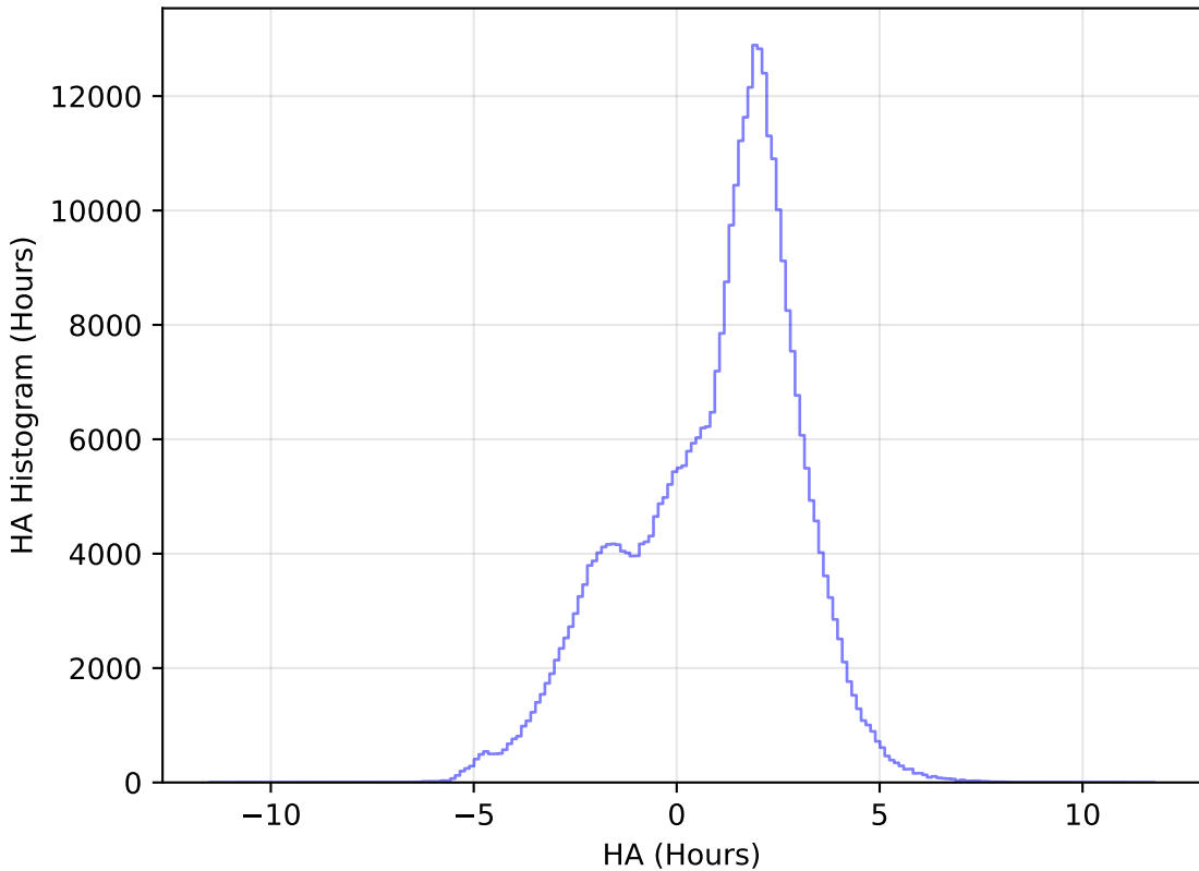
ddf_loaded_fl15_v3.4_10yrs WFD y band: HA Histogram
