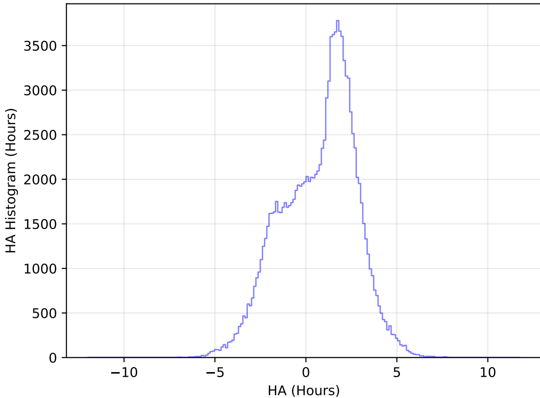
ddf_loaded_fl15_v3.4_10yrs WFD u band: HA Histogram
