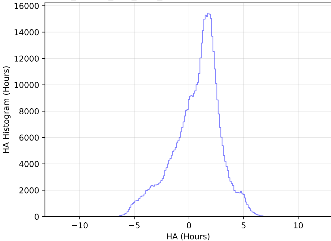
ddf_loaded_fl15_v3.4_10yrs WFD i band: HA Histogram
