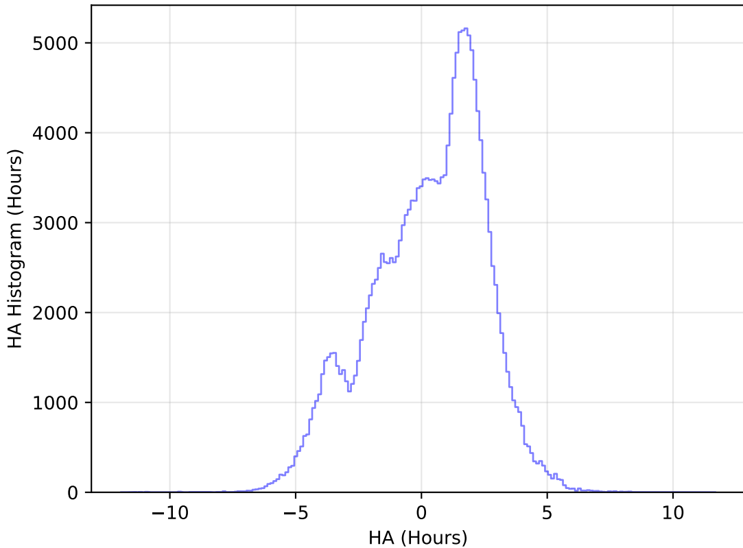
ddf_loaded_fl15_v3.4_10yrs WFD g band: HA Histogram
