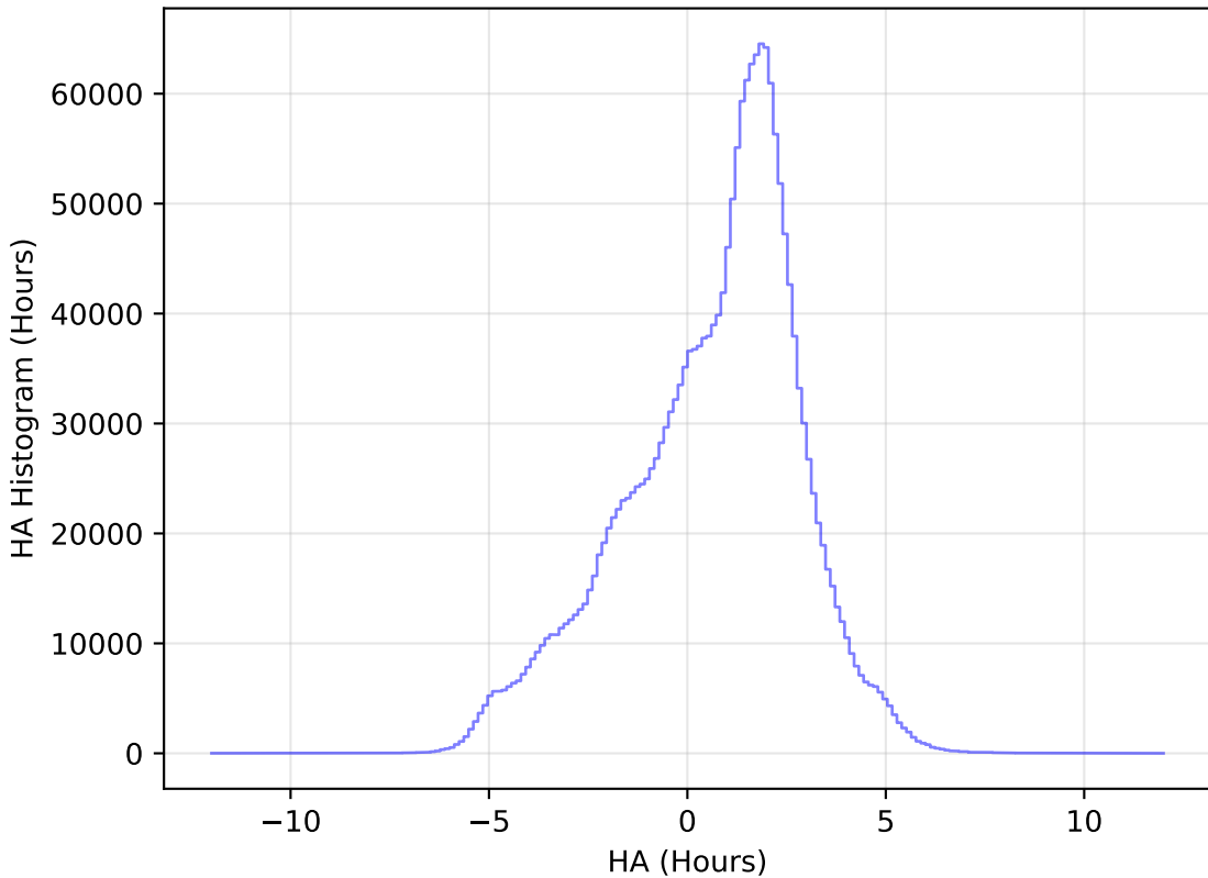
ddf_loaded_fl15_v3.4_10yrs WFD all bands: HA Histogram
