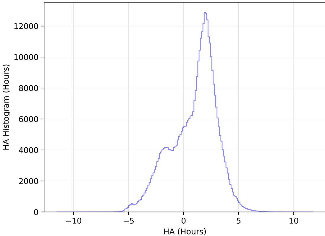
ddf_loaded_fl15_v3.4_10yrs All sky y band: HA Histogram
