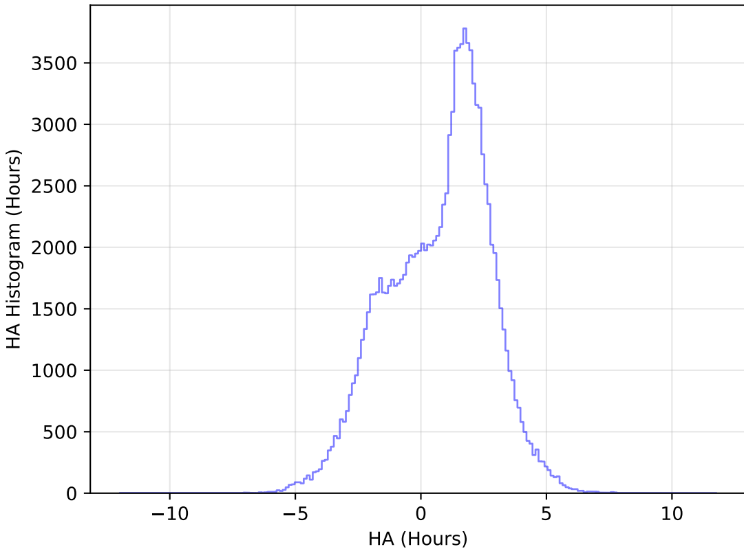
ddf_loaded_fl15_v3.4_10yrs All sky u band: HA Histogram
