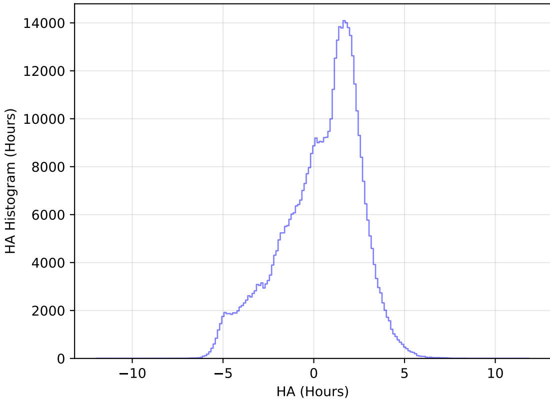
ddf_loaded_fl15_v3.4_10yrs All sky r band: HA Histogram
