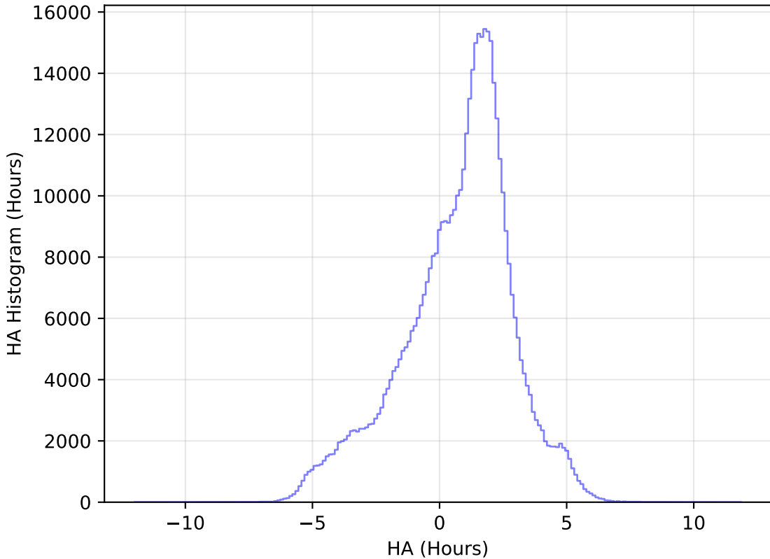
ddf_loaded_fl15_v3.4_10yrs All sky i band: HA Histogram
