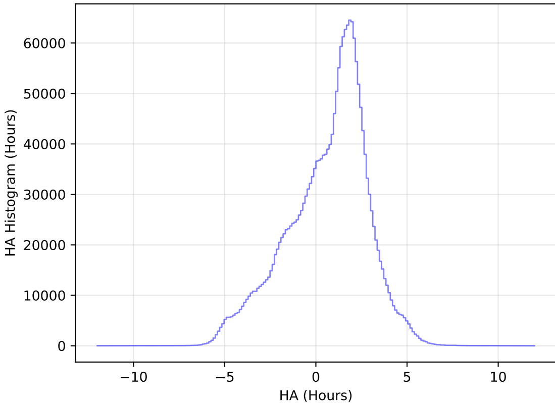
ddf_loaded_fl15_v3.4_10yrs All sky all bands: HA Histogram
