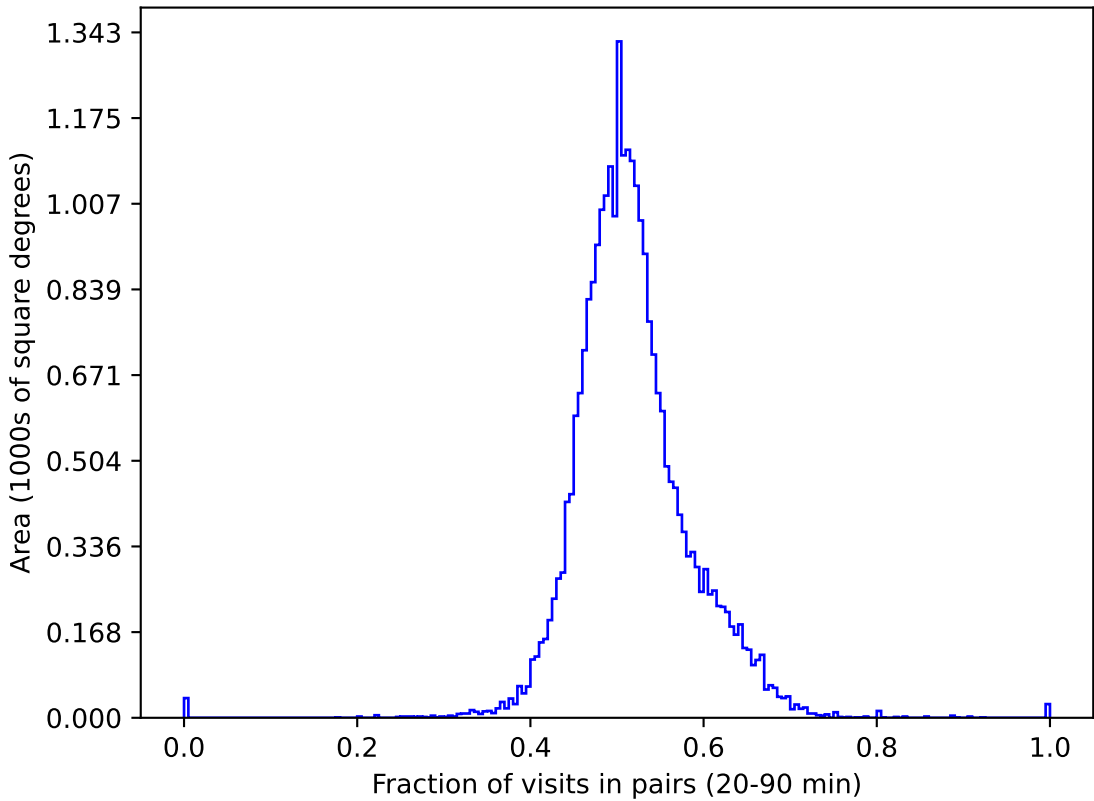
ddf_loaded_fl15_v3.4_10yrs gri All sky: Fraction of visits in pairs (20-90 min)
