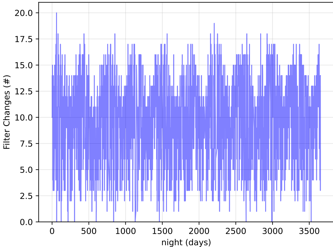
ddf_loaded_fl15_v3.4_10yrs Per Night: Filter Changes
