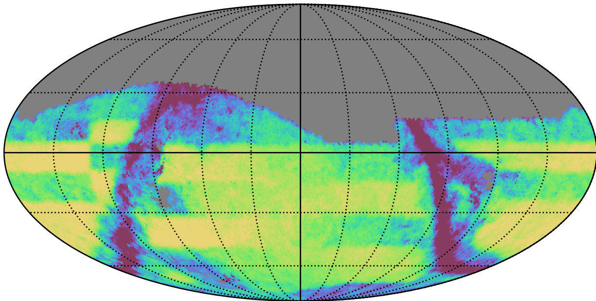
ddf_loaded_fl15_v3.4_10yrs Yr 3-4 i band: Exgal_CoaddM5
