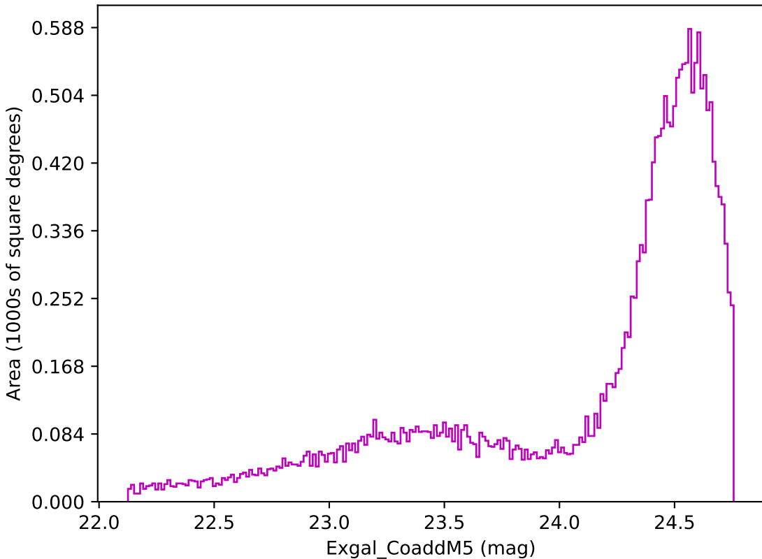
ddf_loaded_fl15_v3.4_10yrs Yr 1 z band: Exgal_CoaddM5
