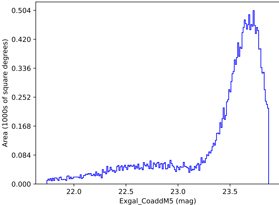
ddf_loaded_fl15_v3.4_10yrs Yr 1 y band: Exgal_CoaddM5
