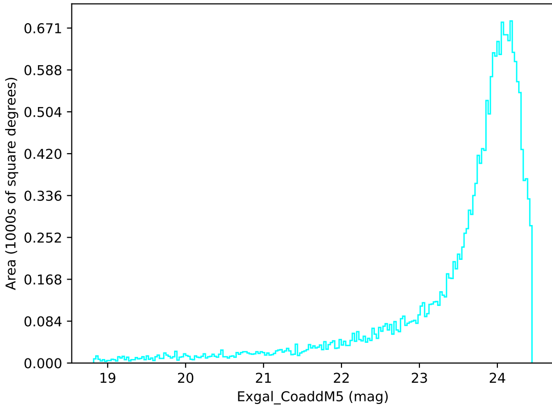
ddf_loaded_fl15_v3.4_10yrs Yr 1 u band: Exgal_CoaddM5
