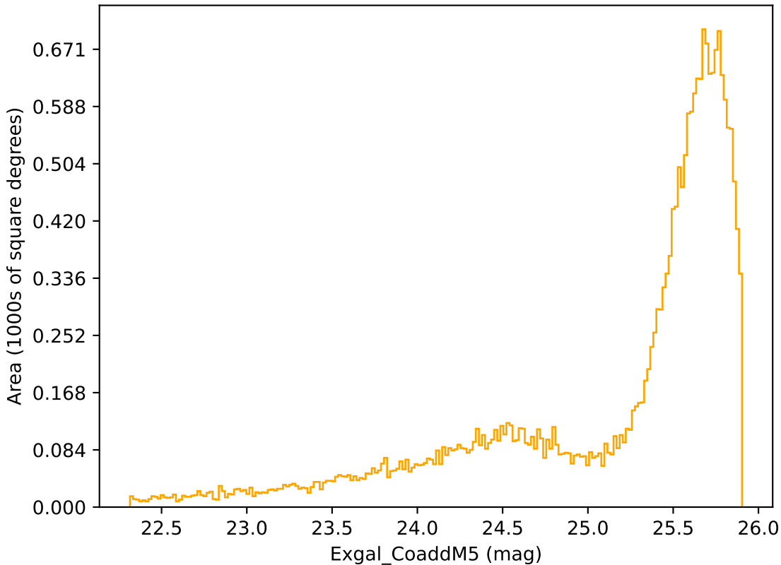
ddf_loaded_fl15_v3.4_10yrs Yr 1 r band: Exgal_CoaddM5
