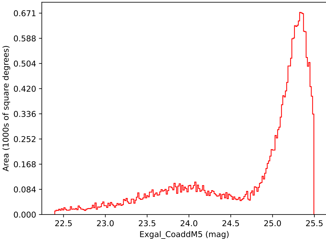
ddf_loaded_fl15_v3.4_10yrs Yr 1 i band: Exgal_CoaddM5
