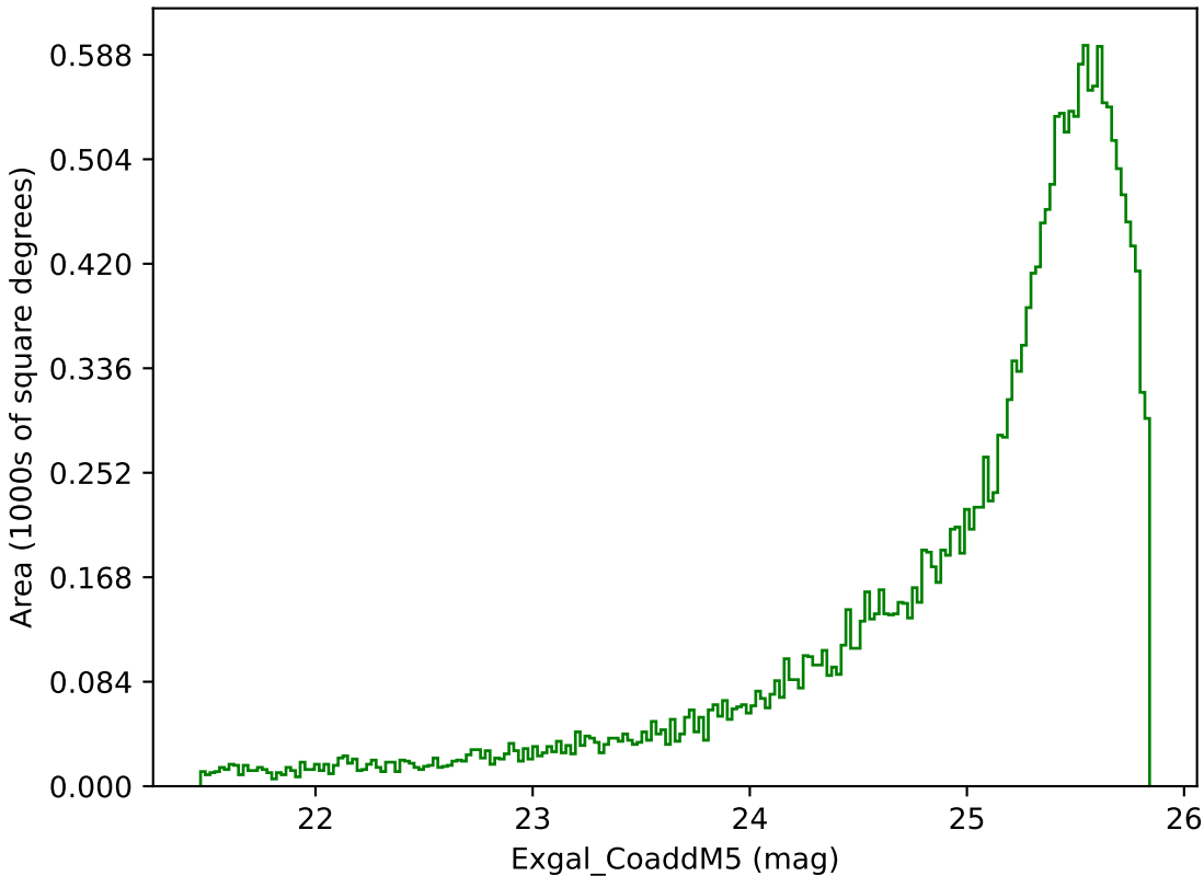
ddf_loaded_fl15_v3.4_10yrs Yr 1 g band: Exgal_CoaddM5
