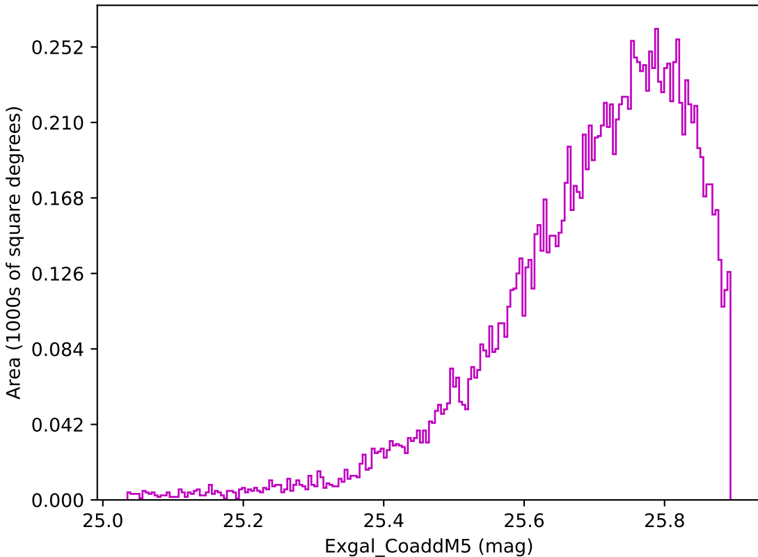
ddf_loaded_fl15_v3.4_10yrs WFD z band: Exgal_CoaddM5
