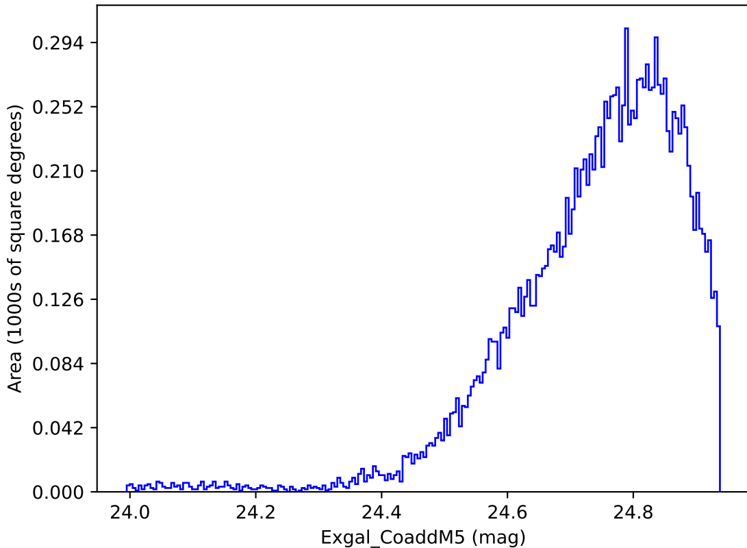
ddf_loaded_fl15_v3.4_10yrs WFD y band: Exgal_CoaddM5
