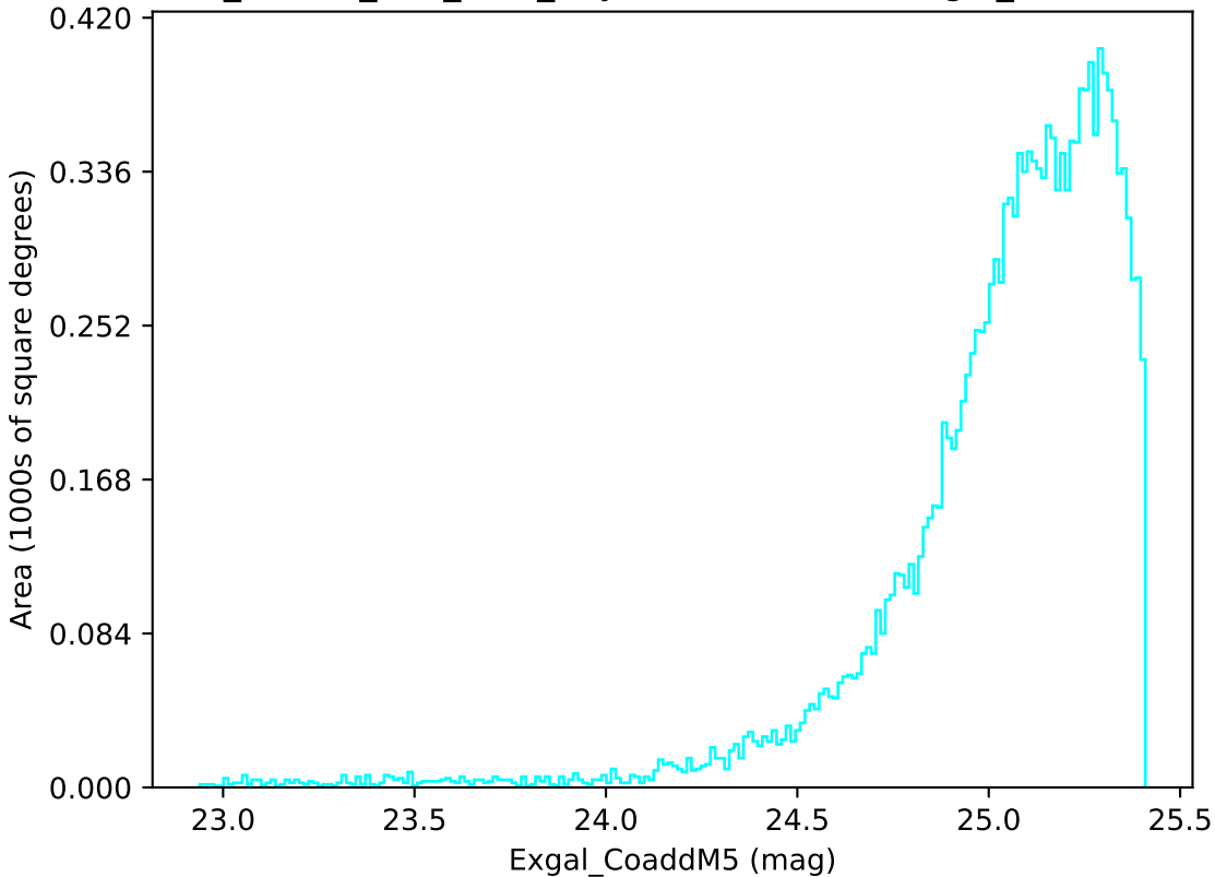
ddf_loaded_fl15_v3.4_10yrs WFD u band: Exgal_CoaddM5
