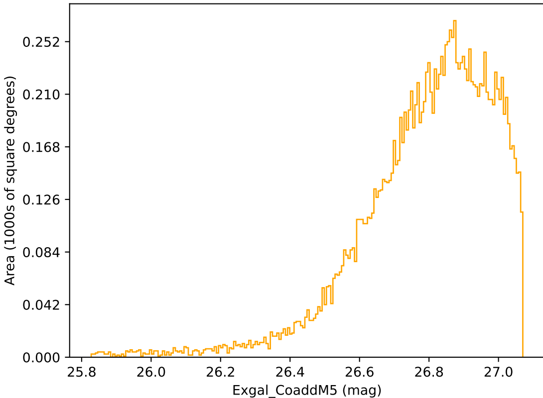
ddf_loaded_fl15_v3.4_10yrs WFD r band: Exgal_CoaddM5
