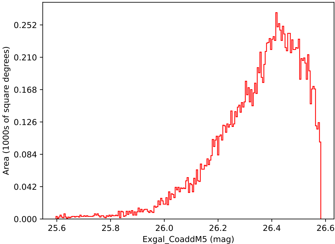
ddf_loaded_fl15_v3.4_10yrs WFD i band: Exgal_CoaddM5
