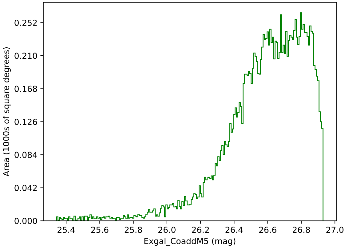
ddf_loaded_fl15_v3.4_10yrs WFD g band: Exgal_CoaddM5
