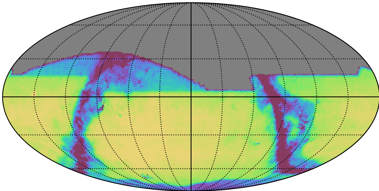
ddf_loaded_fl15_v3.4_10yrs All sky z band: Exgal_CoaddM5
