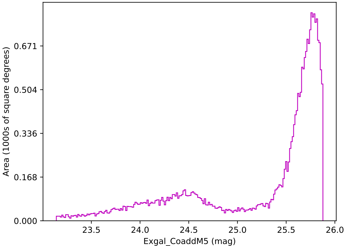
ddf_loaded_fl15_v3.4_10yrs All sky z band: Exgal_CoaddM5
