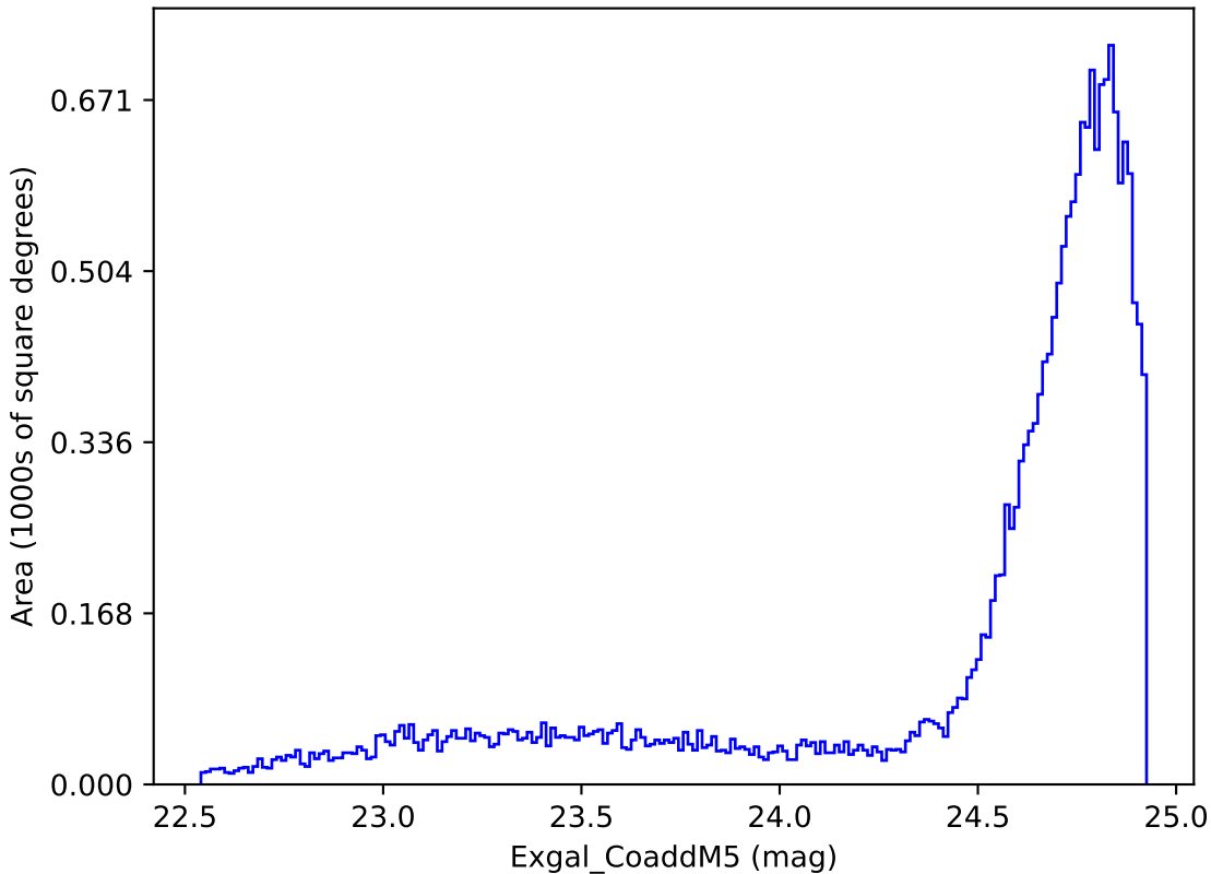
ddf_loaded_fl15_v3.4_10yrs All sky y band: Exgal_CoaddM5
