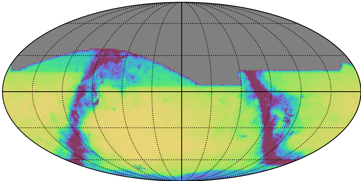
ddf_loaded_fl15_v3.4_10yrs All sky r band: Exgal_CoaddM5
