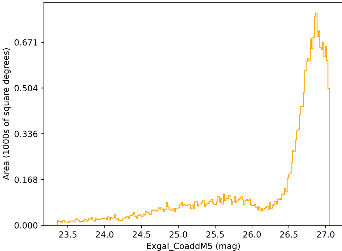
ddf_loaded_fl15_v3.4_10yrs All sky r band: Exgal_CoaddM5
