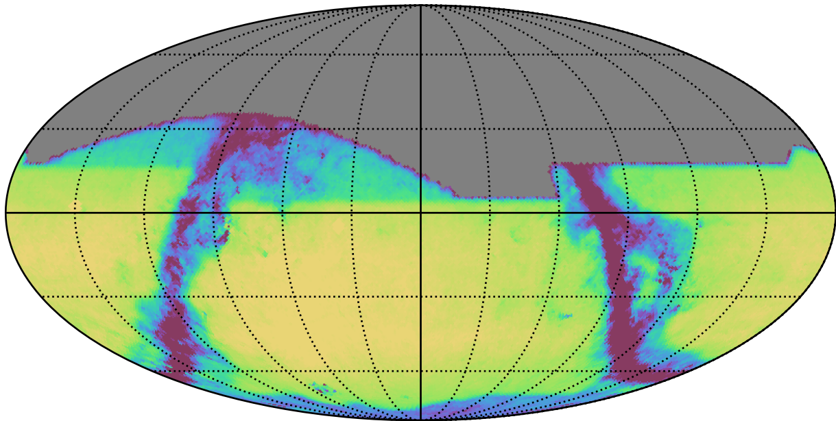
ddf_loaded_fl15_v3.4_10yrs All sky i band: Exgal_CoaddM5
