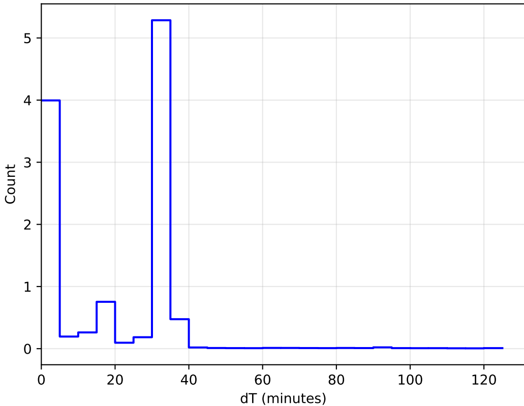
1e6 ddf_loaded_fl15_v3.4_10yrs WFD: DeltaT Histogram
