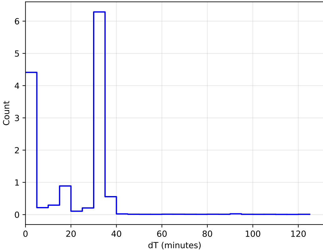
ddf_loaded_fl15_v3.4_10yrs All sky: DeltaT Histogram
